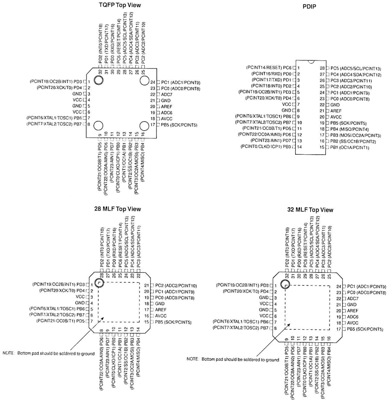
Figure 1-1. Pinout ATmega48/88/1682545M
